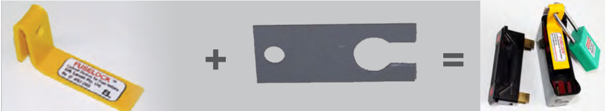
Lockout Base Four different basic shapes/types available. To be permanently attached to the fuse holder.
